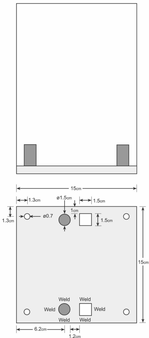
Target Base (plan view)
