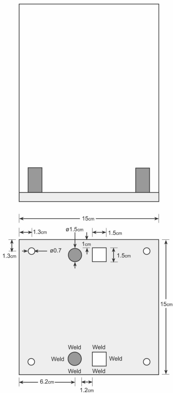
Target Base (plan view)
